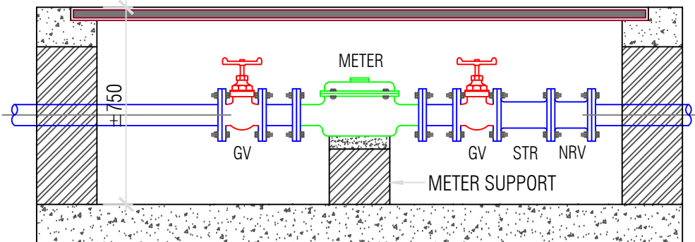
SECTION @ A WATER METER CHAMBER DETAILS SCALE 1:25
